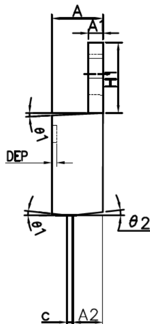
COMMON DIMENSIONS
